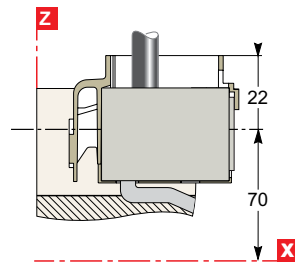
NSX400/630
